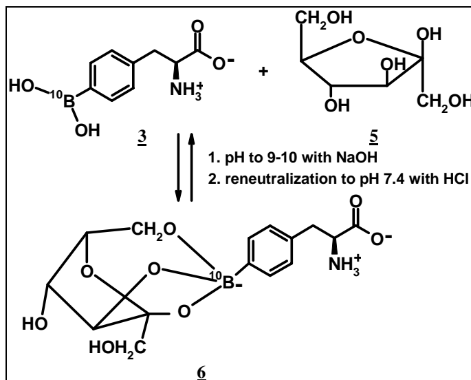
Figure 4. Formulation of anionic BPA-F for in vivo administration schematically: 5 β-furanose ring of fructose and 6 the plausible structure of BPA-F (Shull et al. 2000)
